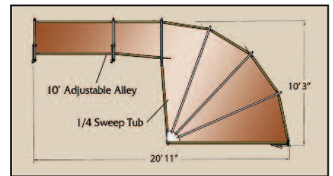
PRXL7 Tub and Alley Package Order No. 010-50100 2-inch Tube, 72-inch High
